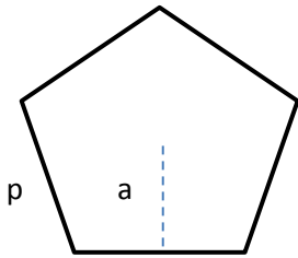
Regular polygon
