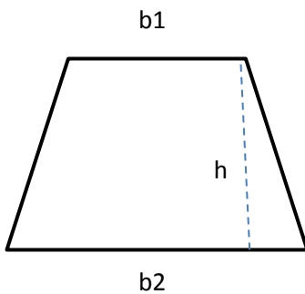
Trapezoid
