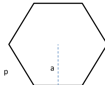
Regular polygon
